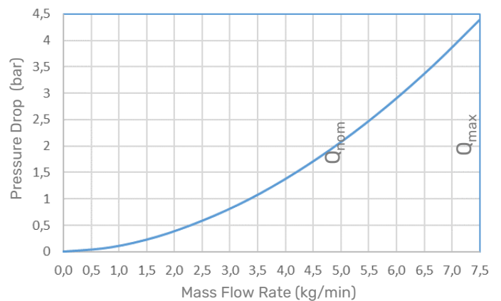
0 – 7.5 kg/min water, sensor with P1 pressure rating. Higher viscosities create higher pressure drop
