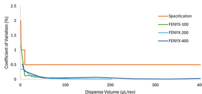
Dispense Volume vs. Precision
