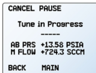
Optimize Control in progress.
